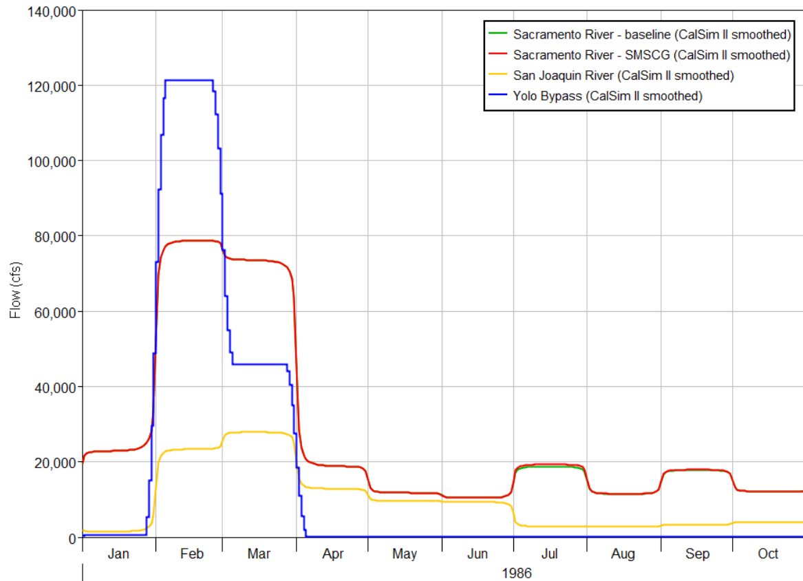
Figure 57 Major inflows for the Wet (1986 CS) scenario simulations. Sacramento River inflows differ slightly at times for SMSCG scenario simulations.
